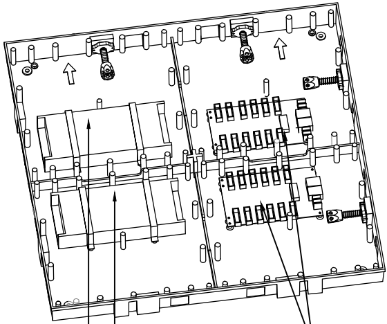
POWER SUPPLY
